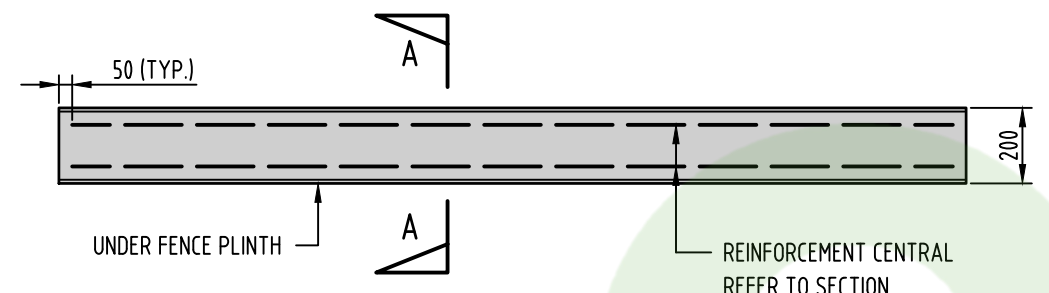
ELEVATION VIEW SCALE 1:20
