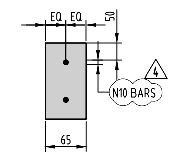
SECTION B-B SCALE 1:10
