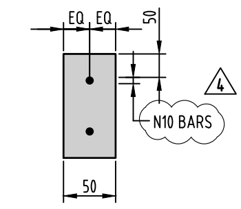
SECTION A-A SCALE 1:10
